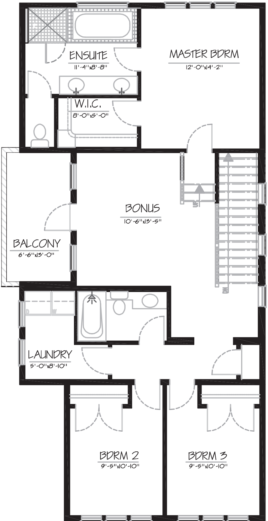
upper floor plan 1,092 sq. ft.
