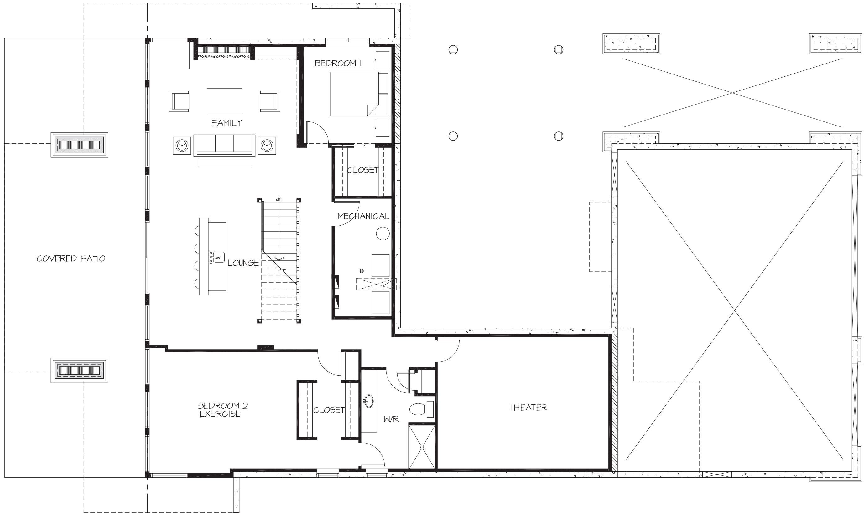
BASEMENT FLOOR PLAN 1489 SQ.FT. TOTAL 4298 SQ.FT.
