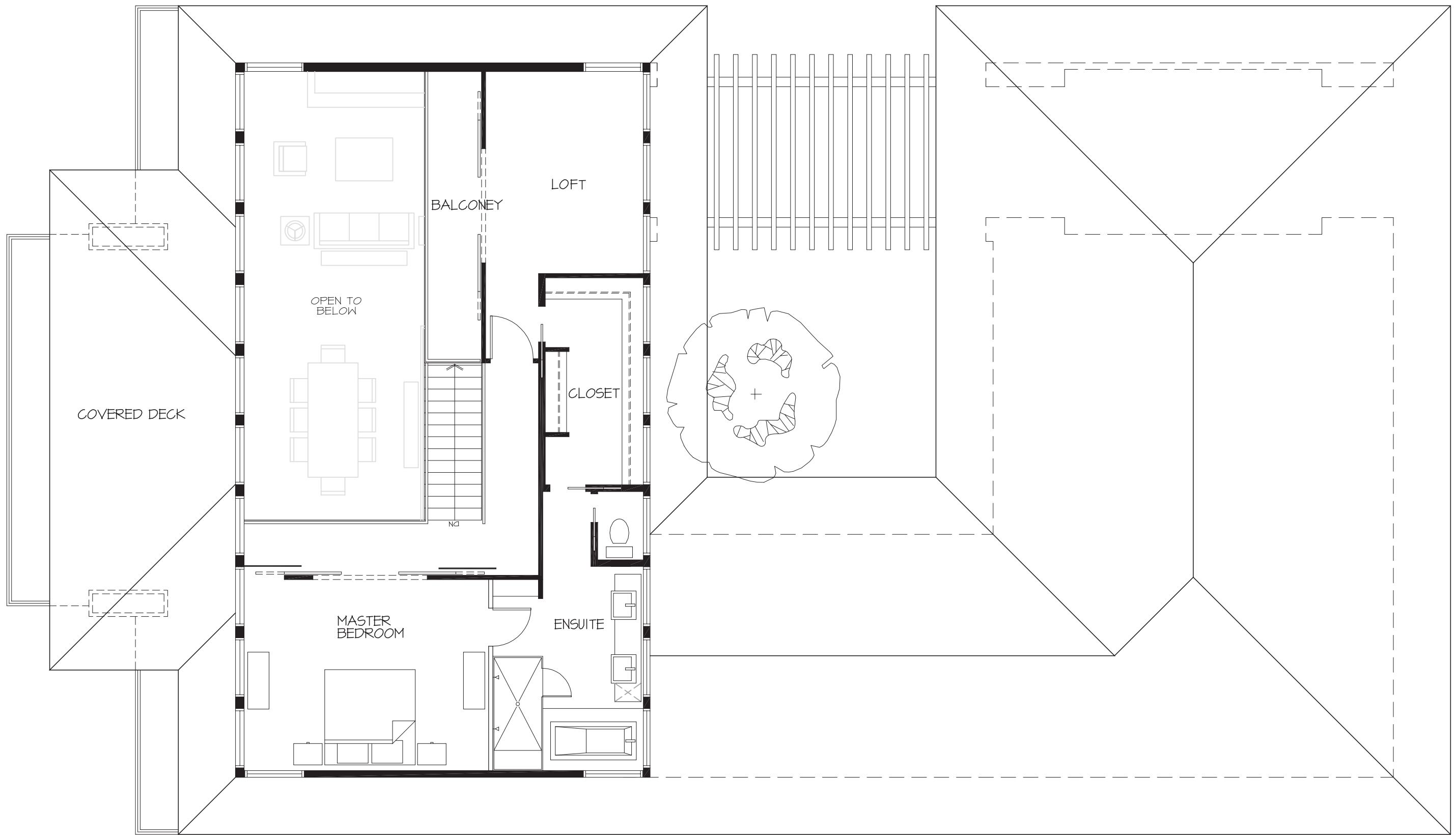
UPPER FLOOR PLAN 984 SQ.FT. TOTAL 4298 SQ.FT
