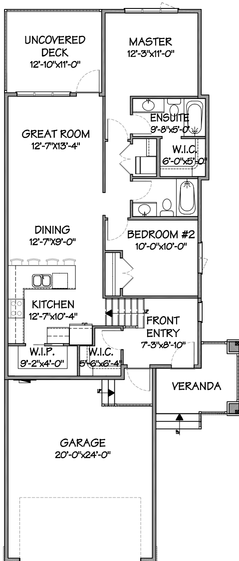
MAIN LEVEL FLOOR PLAN 1,124 FT2
