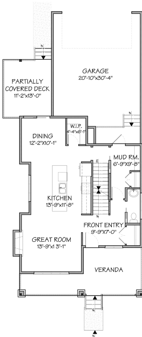
MAIN LEVEL FLOOR PLAN 834 FT 2
