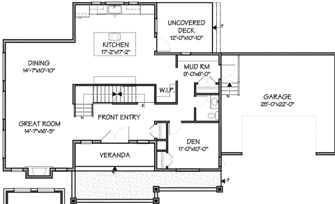
MAIN LEVEL 1,334 FT 2
