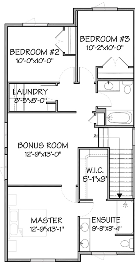
UPPER LEVEL FLOOR PLAN 963 FT 2
