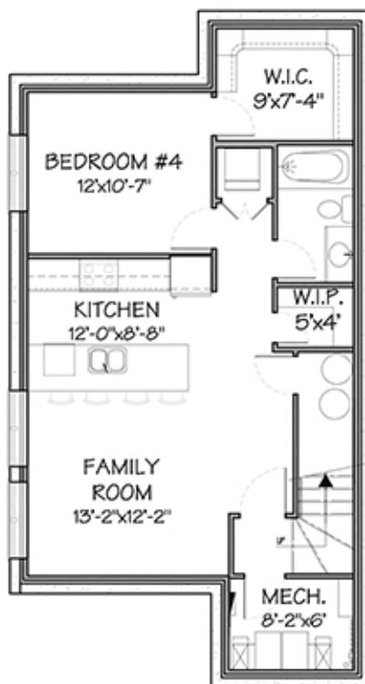
LOWER LEVEL LEGAL SUITE 690 FT 2
